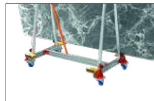
4 swivel castors with brakes equipped with wood damping supports
